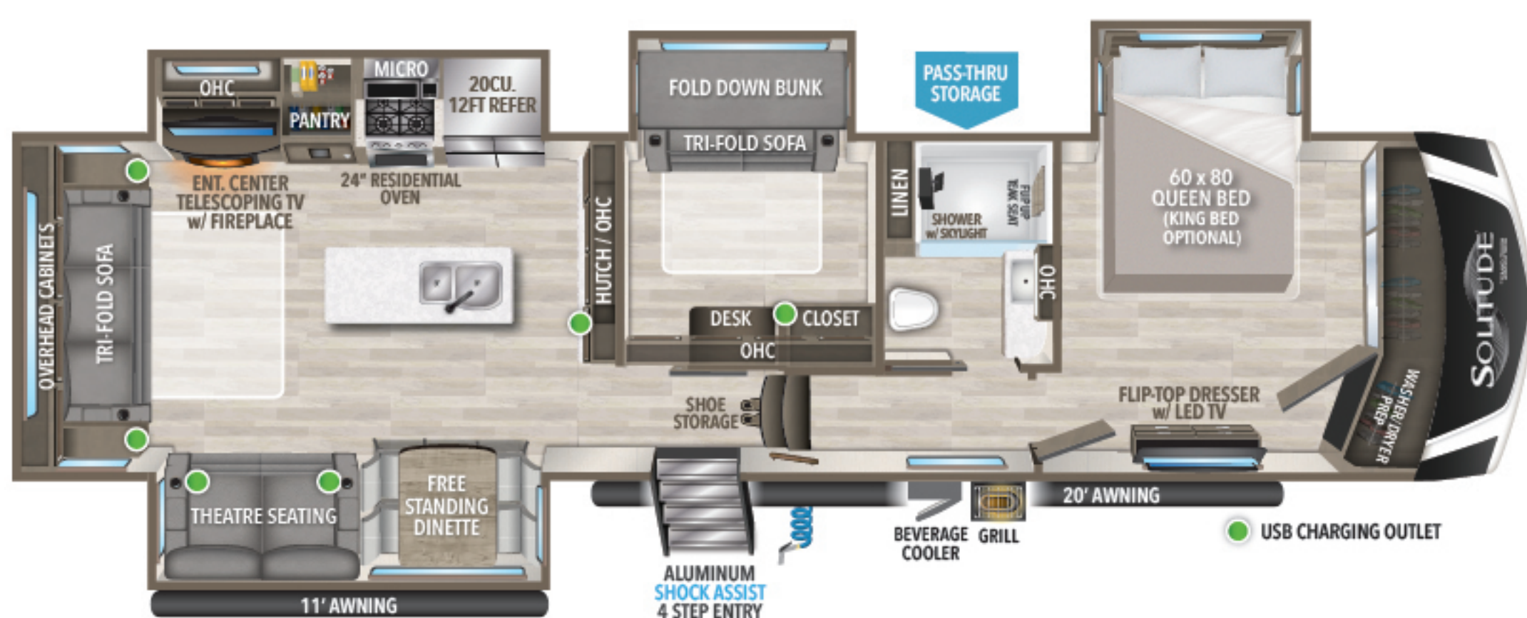
378MBS UVW † 14,344 HITCH ‡ 2,686 GVWR 16,800 LENGTH ‡ 40' 2" HEIGHT 13' 5" CAPACITY 81 106 53
