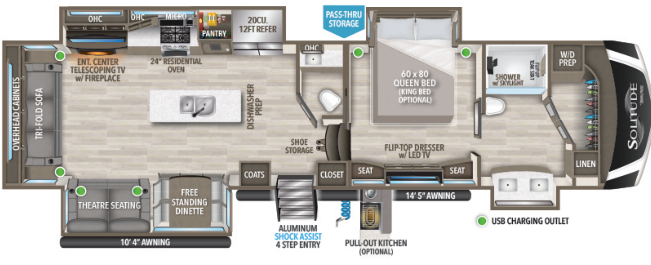
373FB UVW † 13,950 HITCH ‡ 2,800 GVWR 16,800 LENGTH ‡ 41' 4" HEIGHT 13' 5" CAPACITY 81 106 106
