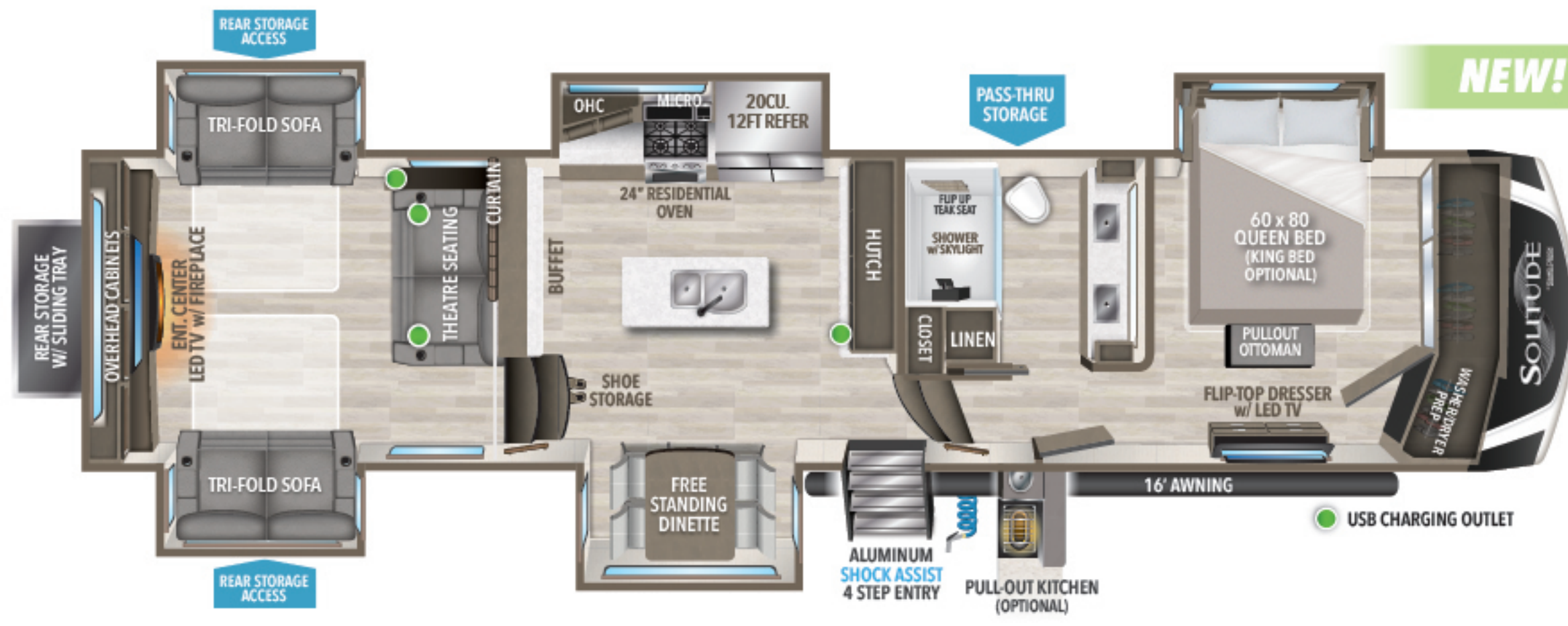
376RD UVW † TBD HITCH ‡ TBD GVWR 16,800 LENGTH ‡ 42' 6" HEIGHT 13' 5" CAPACITY 81 106 53
