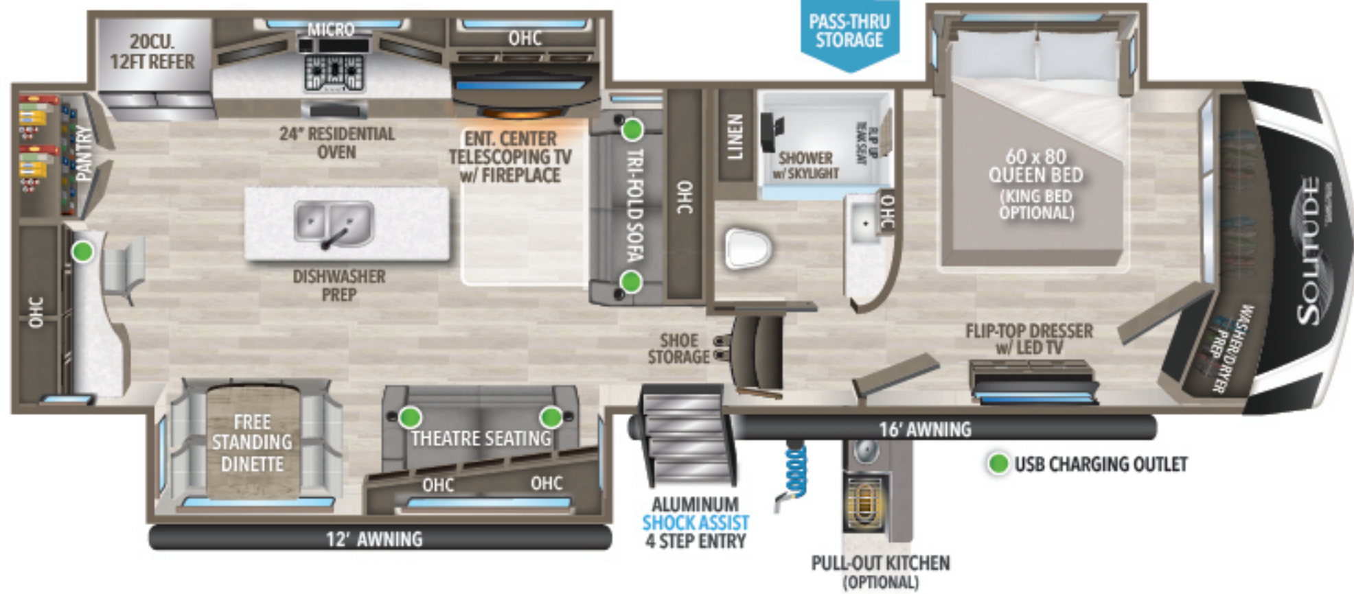
345GK UVW † 13,320 HITCH ‡ 2,604 GVWR 16,800 LENGTH ‡ 37' 2" HEIGHT 13' 5" CAPACITY 81 106 53
