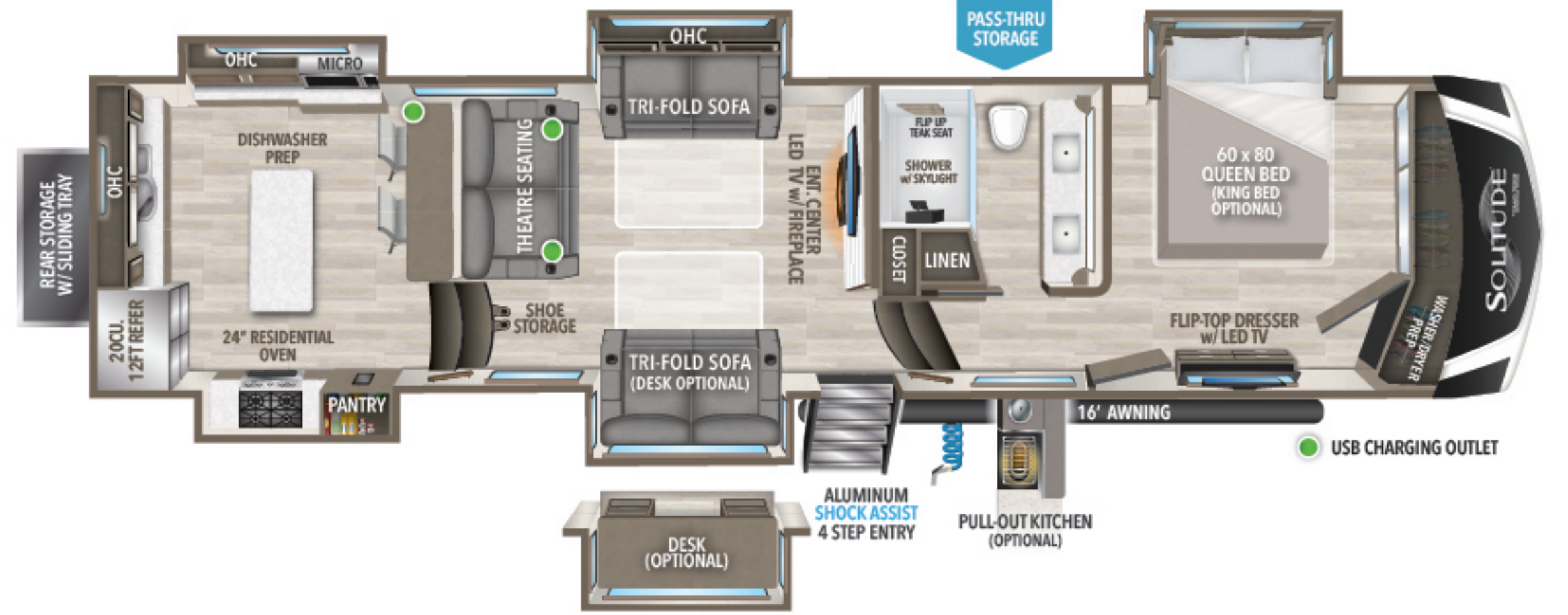
390RK UVW † 14,562 HITCH ‡ 2,794 GVWR 16,800 LENGTH ‡ 41' 5" HEIGHT 13' 5" CAPACITY 81 106 53
