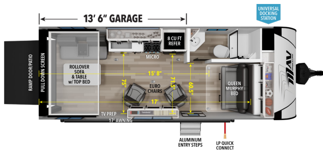
22MAV 13' 6" GARAGE UVW 1 HITCH 1 GVWR LENGTH 2 HEIGHT 3 CAPACITY 5,900 943 9,950 26' 6" 12' 2" 90 74 37
