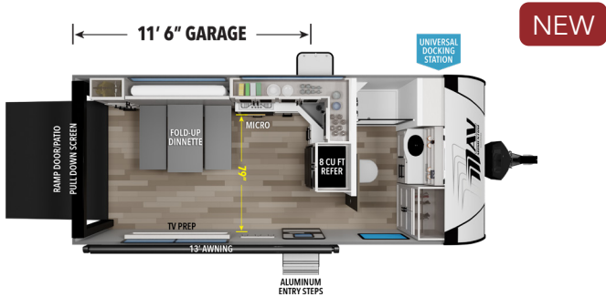
17MAV 11' 6" GARAGE UVW 1 HITCH 1 GVWR LENGTH 2 HEIGHT 3 CAPACITY 5,542 873 9,950 22' 11" 12' 2" 90 74 37
