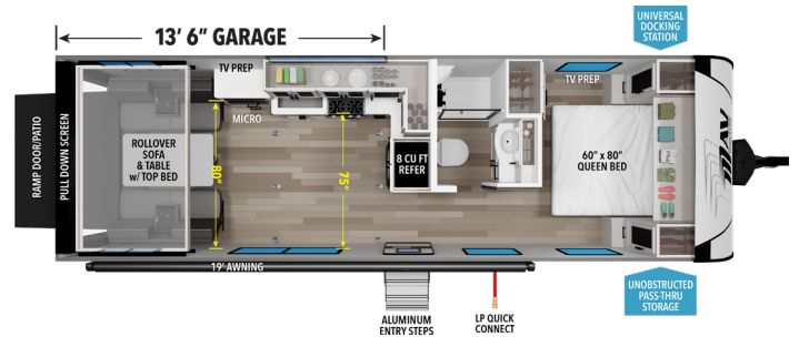
27MAV 13' 6" GARAGE UVW 1 HITCH 1 GVWR LENGTH 2 HEIGHT 3 CAPACITY 6,900 1,187 11,000 32' 2" 12' 2" 90 74 37
