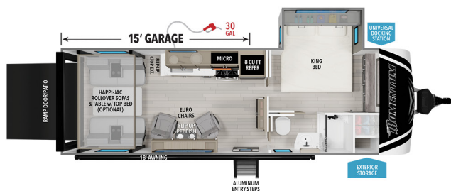
23G 15' GARAGE UVW 1 EMPTY HITCH 1 GVWR LENGTH 1 HEIGHT CAPACITY 7,669 1,242 13,000 28' 10" 12' 4" 90 74 39
